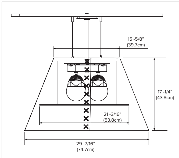
Elevation View
