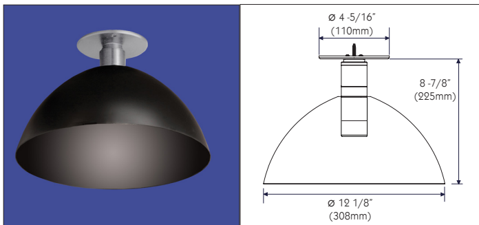
Kore-EX5 LED, Monopoint, Frosted Cylinder Gem, Bolle Shade Kore-EX5: Aluminum or Black Finish; Bolle Shade: Black Finish
