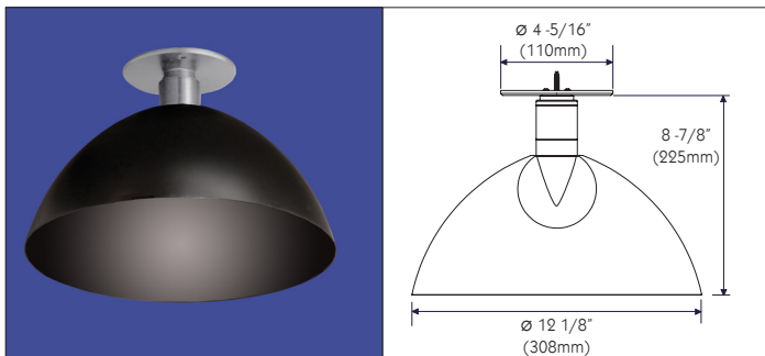
Kore-EX5 LED, Monopoint, Frosted Sphere Gem, Bolle Shade Kore-EX5: Aluminum or Black Finish; Bolle Shade: Black Finish
