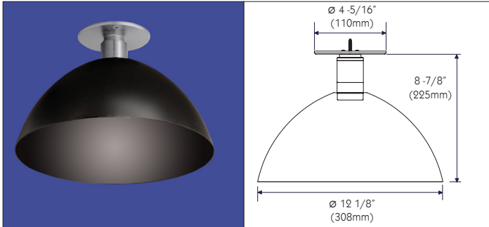
Kore-EX5 LED, Monopoint, Flat Gem, Bolle Shade Kore-EX5: Aluminum or Black Finish; Bolle Shade: Black Finish
