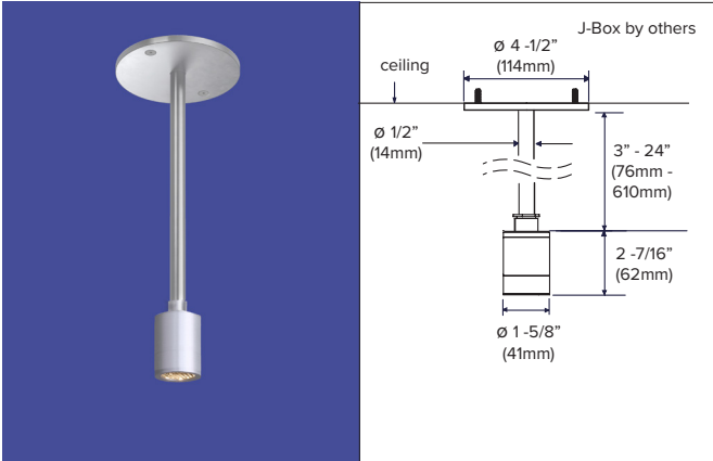
Kore EX5 Stem Pendant Monopoint with Downlight, Remote Power Supply, shorter rigid pendant length shown. 24" Field-cutable rigid stem, 3" length minimum.
