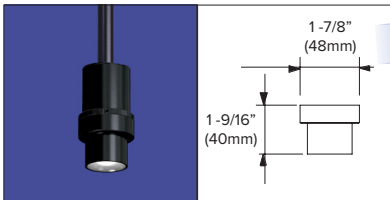
Exton Snoot (EX5-SNT-BLK)
